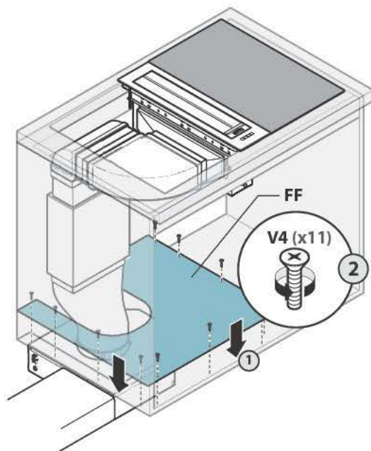
INSTALLAZIONE A PARETE CAPP A PIANO DOUBLE SUCTION PIANO DOUBLE SUCTION HOOD WALL INSTALLATION
