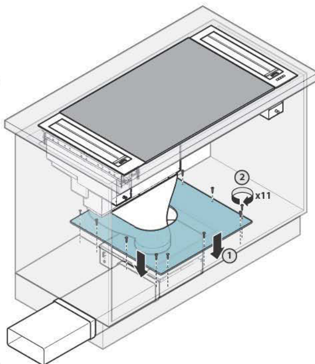
INSTALLAZIONE A PARETE CAPP A PIANO DOUBLE SUCTION PIANO DOUBLE SUCTION HOOD WALL INSTALLATION
