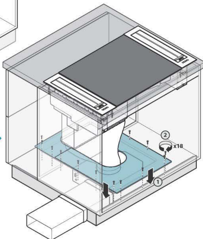
INSTALLAZIONE A ISOLA CAPP A PIANO DOUBLE SUCTION PIANO DOUBLE SUCTION HOOD ISLAND INSTALLATION
